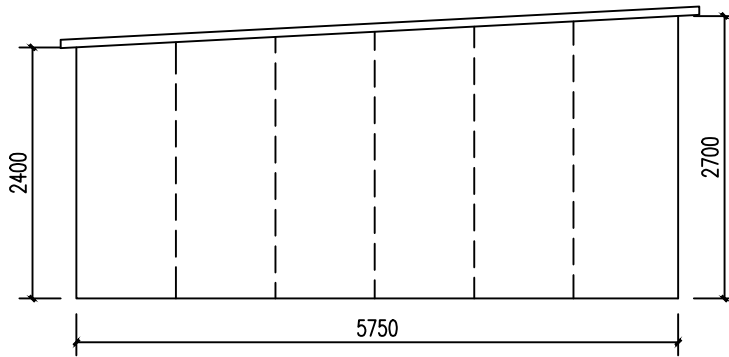
50m 2 Left 1:50
