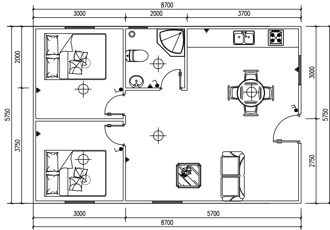
50m 2 Layout 1:50
