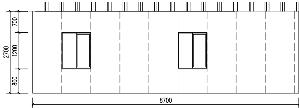
50m 2 Front 1:50
