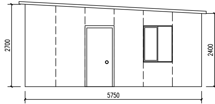
50m 2 Right 1:50
