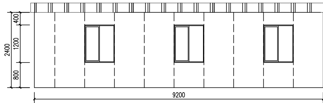
70m 2 Rear 1:50
