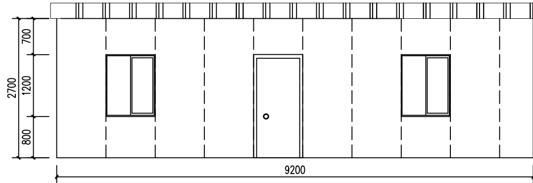
70m 2 Front 1:50
