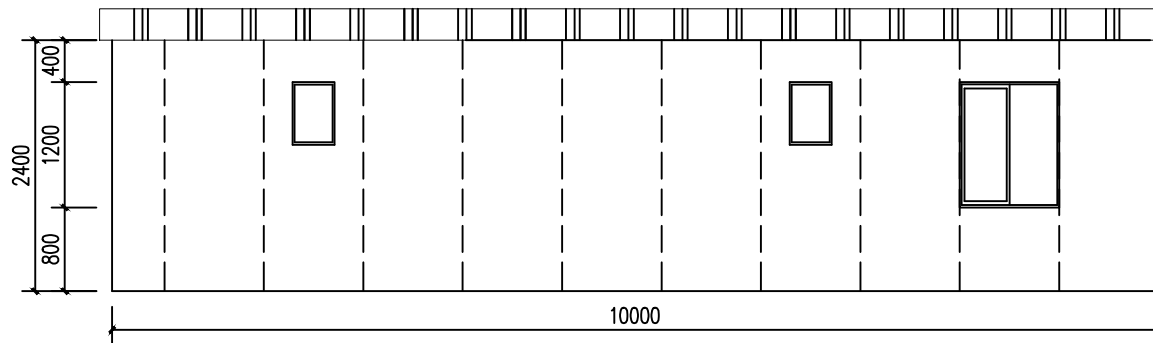
60m 2 Rear 1:50
