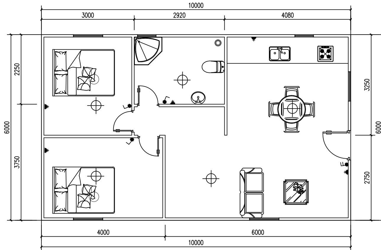
60m 2 Layout 1:50
