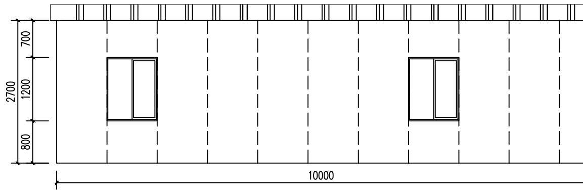
60m 2 Front 1:50
