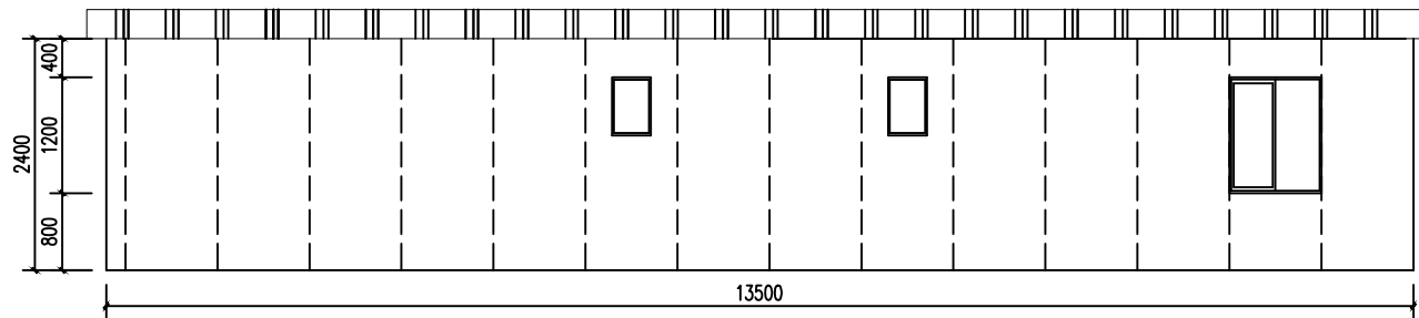
100m 2 Rear 1:50
