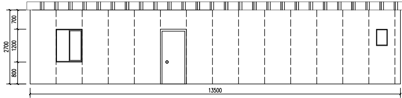
100m 2 Front 1:50
