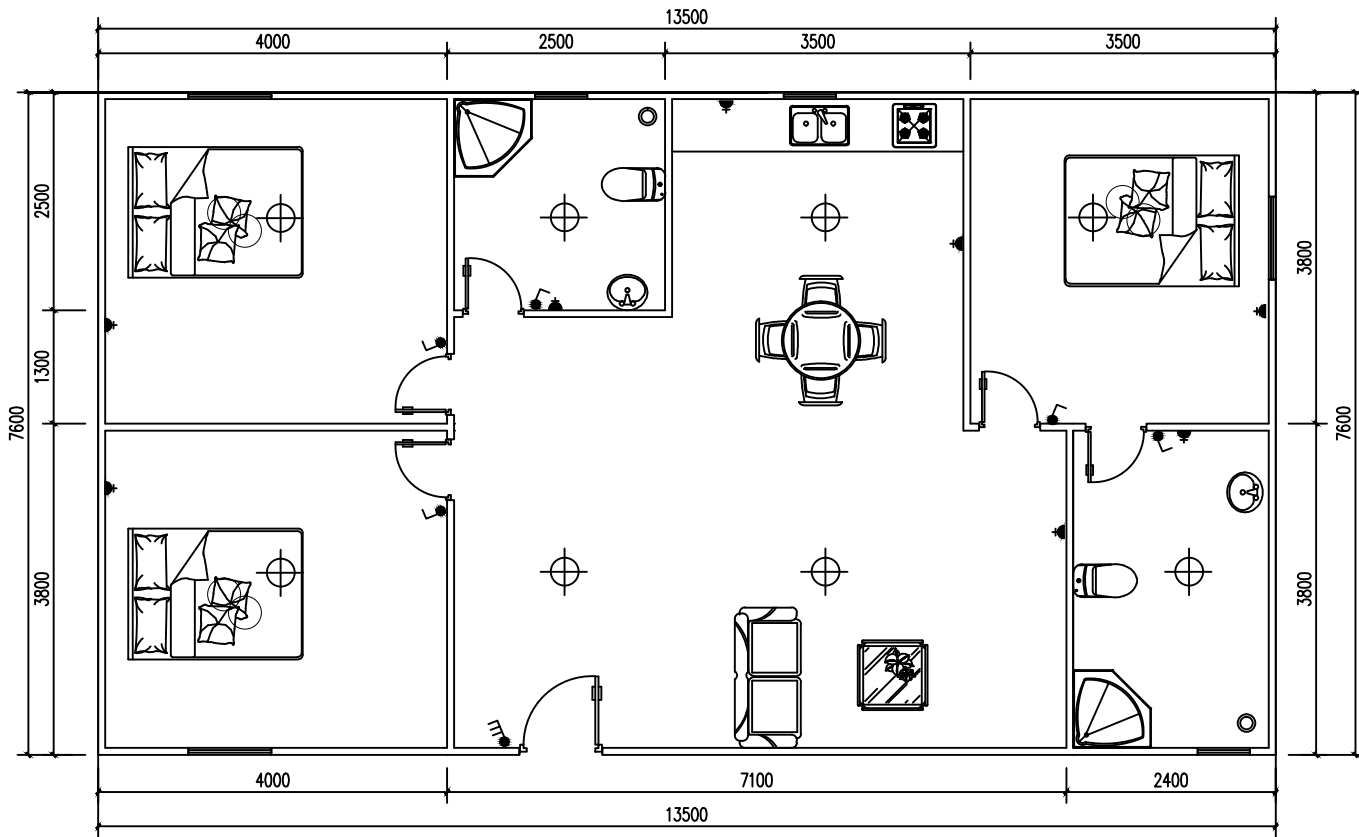
100m 2 Layout 1:50
